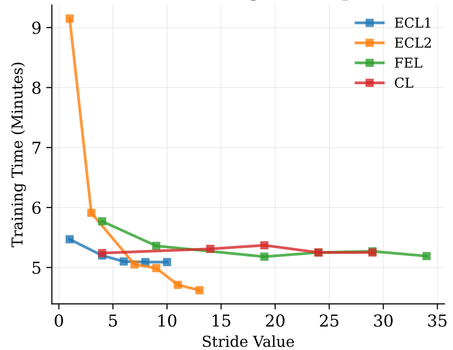
Stride: Training Time Impact
