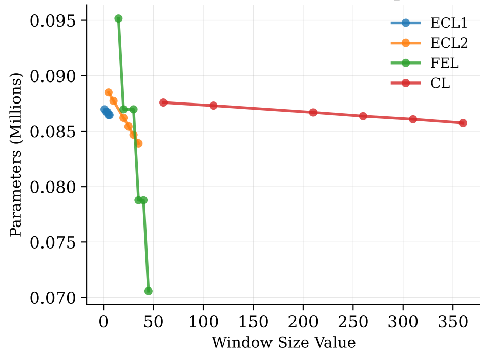
Window Size: Model Size Impact
