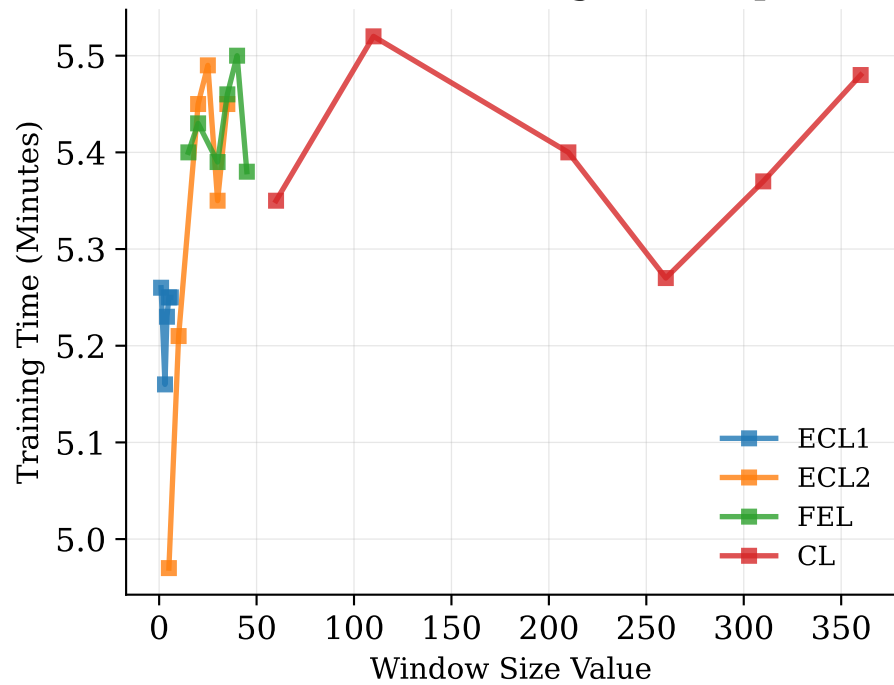
Window Size: Training Time Impact
