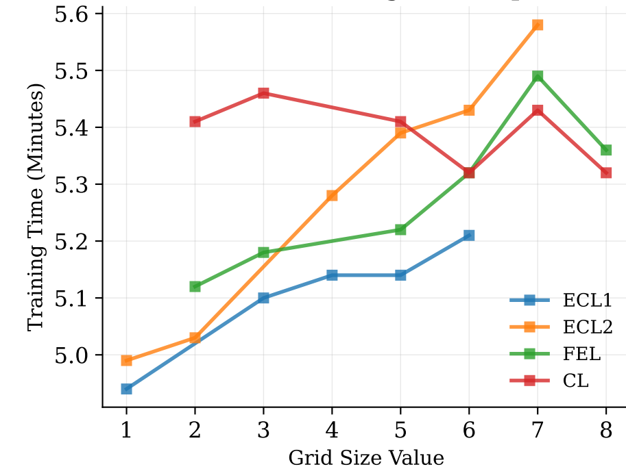
Grid Size: Training Time Impact
