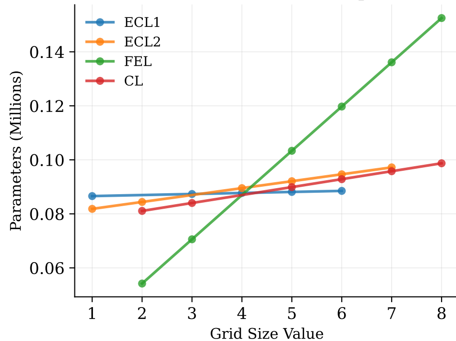
Grid Size: Model Size Impact
