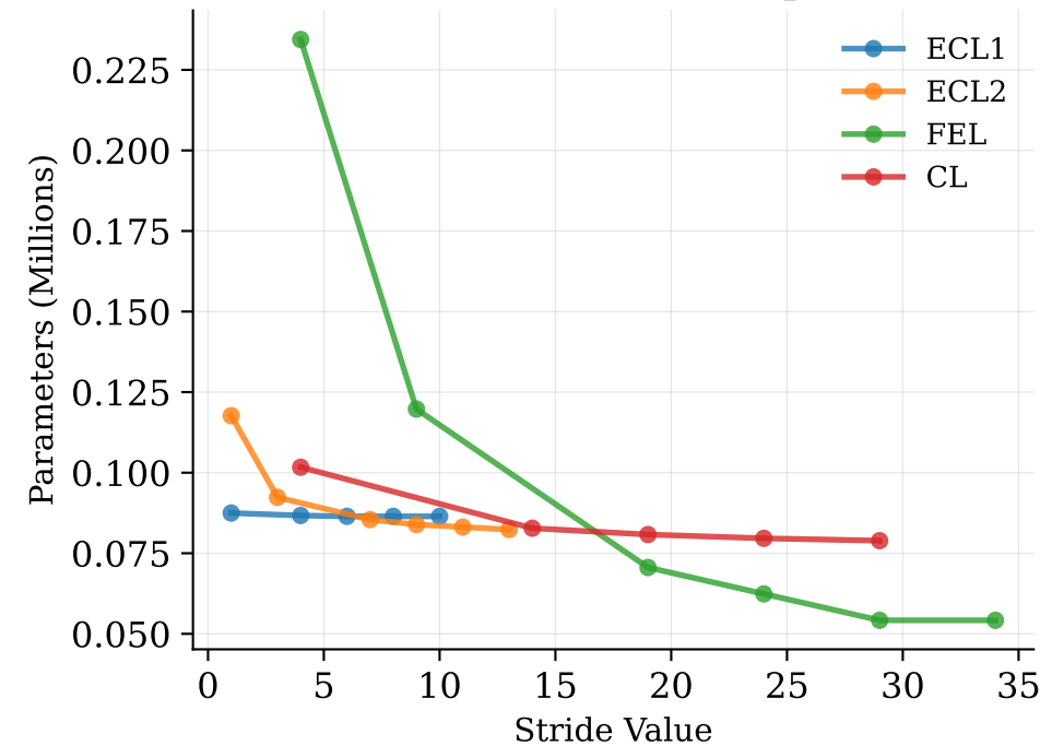
Stride: Model Size Impact
